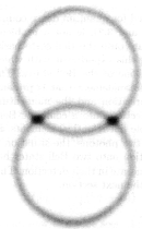
FIG. 4: Type-II down-conversion light as seen through a narrow-band filter. The two rings are the ordinary and extraordinary cones of light rays. Along the intersecting directions, which are cut out by irises, we observe unpolarized light.
